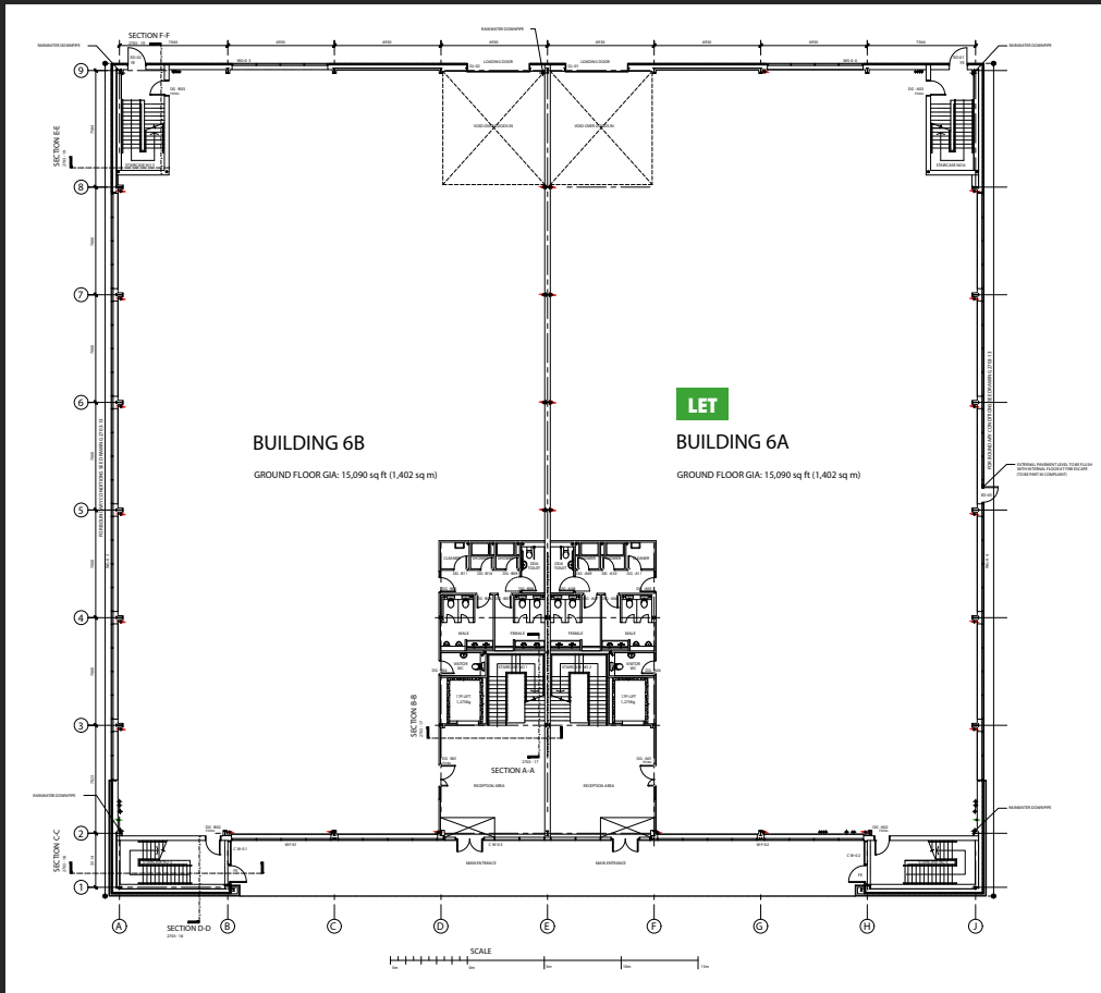
BUILDING 6 GROUND FLOOR PLAN SCALE 1 : 125
