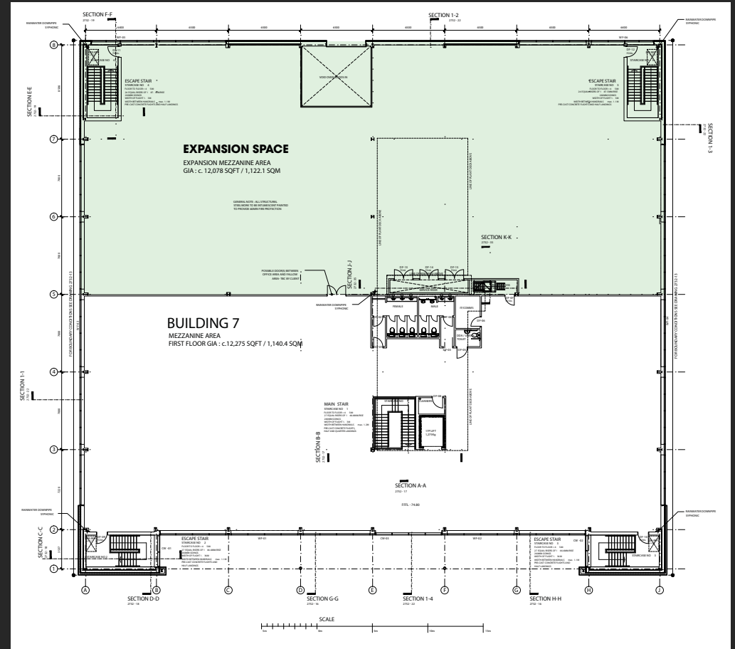
BUILDING 7 FIRST FLOOR PLAN SCALE 1 : 100
